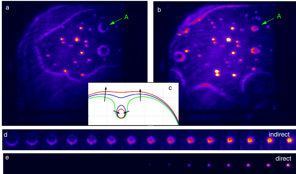
Figure 17. Shrinkage of exciton rings to localized bright spots at nearly homogeneous excitation: spatial PL pattern for indirect excitons at T = 1.8 K, V_g = 1.15 V, and (a) P_{ex} = 390 \mu W and (b) P_{ex} = 600 \mu W. With (a) and (b), the area of view is 690 \times 590 \mu m. (c) Theoretical electron-hole interface for a point source of holes and a weaker point source of electrons. Arrows show interface displacement at increasing hole number. Note the ring shrinking around the electron source. The shrinkage of ring A (a, b) of indirect excitons is detailed in (d) for T = 380 mK, V_g = 1.155 V and P_{ex} = 77 – 160 \mu W (from left to right) with the defocused excitation spot maximum moved to a location directly below ring A. With (d) and (e), the area of view is 67 \times 67 \mu m for each image. Ring shrinkage is accompanied by the onset of the direct exciton emission (e) indicating hot cores at the centre of the collapsed rings. From [31].
